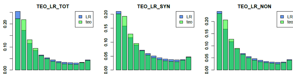
Figure 5.6 Site frequency spectrum (SFS) showing the frequency of alleles in maize landraces (LR) and teosinte parviglumis (teo). Columns to the left represent rare alleles (i.e. those of a low frequency in the population, for the leftmost column that is <0.7 ) and columns to the right represent common alleles (i.e. more frequent in the population, for the rightmost column that is >0.92 ). Panels show the SFS for all sites (_TOT), for synonymous sites (_SYN; when the alternative allele does not change the amino acid that would be produced by the DNA) and for non-synonymous sites (_NON; when a different amino acid, and hence protein, would be produced by that allele). Leftmost columns show that the landraces present more rare alleles than the teosinte. Taken from Hufford et al. (2012).
